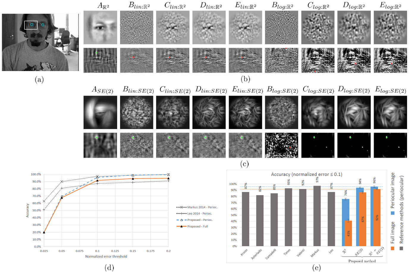
Fig. 5. Overview of trained templates for right-eye pupil detection, and their responses to a challenging image from the BioID database. (a) The example input image with true pupil locations (blue circle with a radius that corresponds to a normalized error threshold of 0.1, see Eq. 39). The white square indicates the periorcular image region for the right eye. (b) The \mathbb{R}^2 -type templates (top row) and their responses to the input image (bottom row). (c) The maximum intensity projections (over \theta ) of the SE(2) -type templates (top row) and their responses to the input image (bottom row). Detected pupil locations are indicated with colored circles (green = correct, red = incorrect, based on a normalized error threshold of 0.1). (d) Accuracy curves generated by varying thresholds on the normalized error, in comparison with the two most recent methods from literature. (e) Accuracy (at a normalized error threshold of 0.1) comparison with pupil detection methods from literature.
